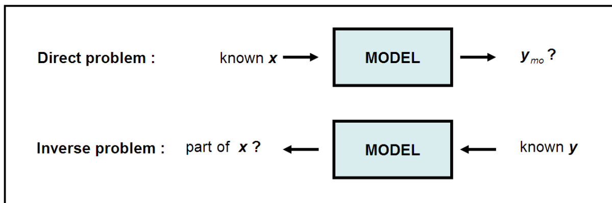
Figure 8. Direct problem/Inverse problem
